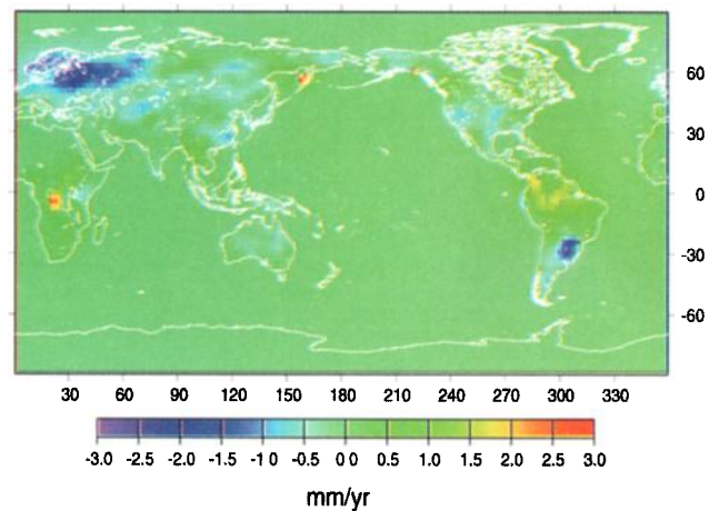
Figure 4. Global distribution of vertical displacement rates (mm/yr) modeled using 3 years (1996-1998) of water-storage data.
